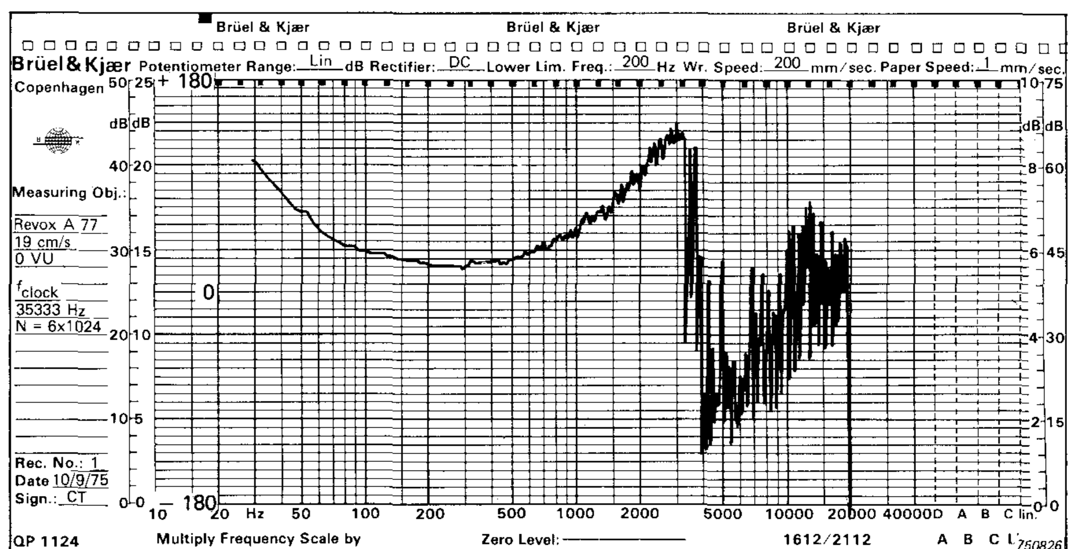
Fig.10. Tape recorder phase measurements using an improperly adjusted clock frequency for the Phase Delay Unit
