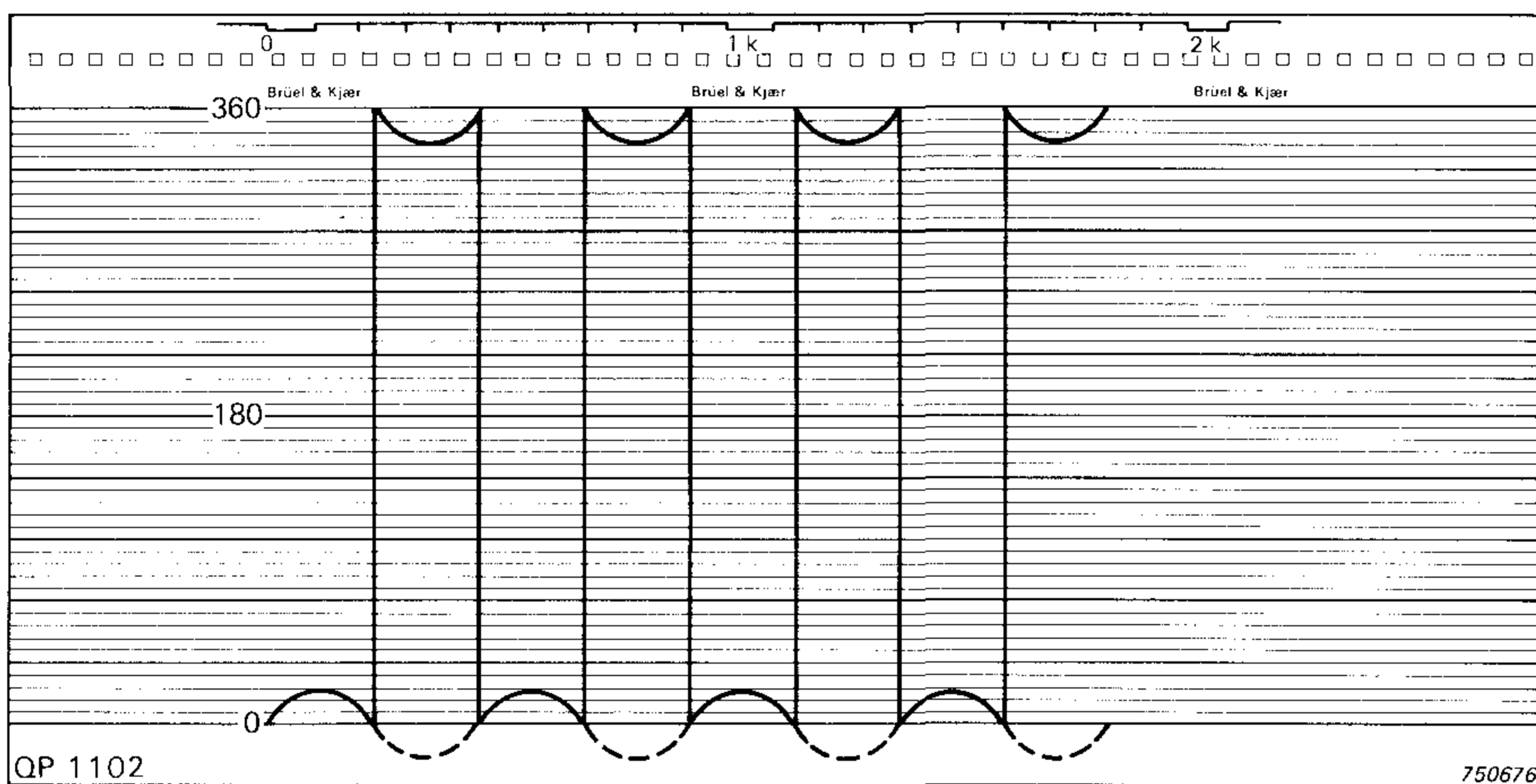
Fig. 16. When the reference is at the bottom line, a phase shift around 0^\circ will shift between just above 0^\circ to just below 360^\circ . By use of one of the slope switches, the 0^\circ reference can be moved to the middle of the paper
