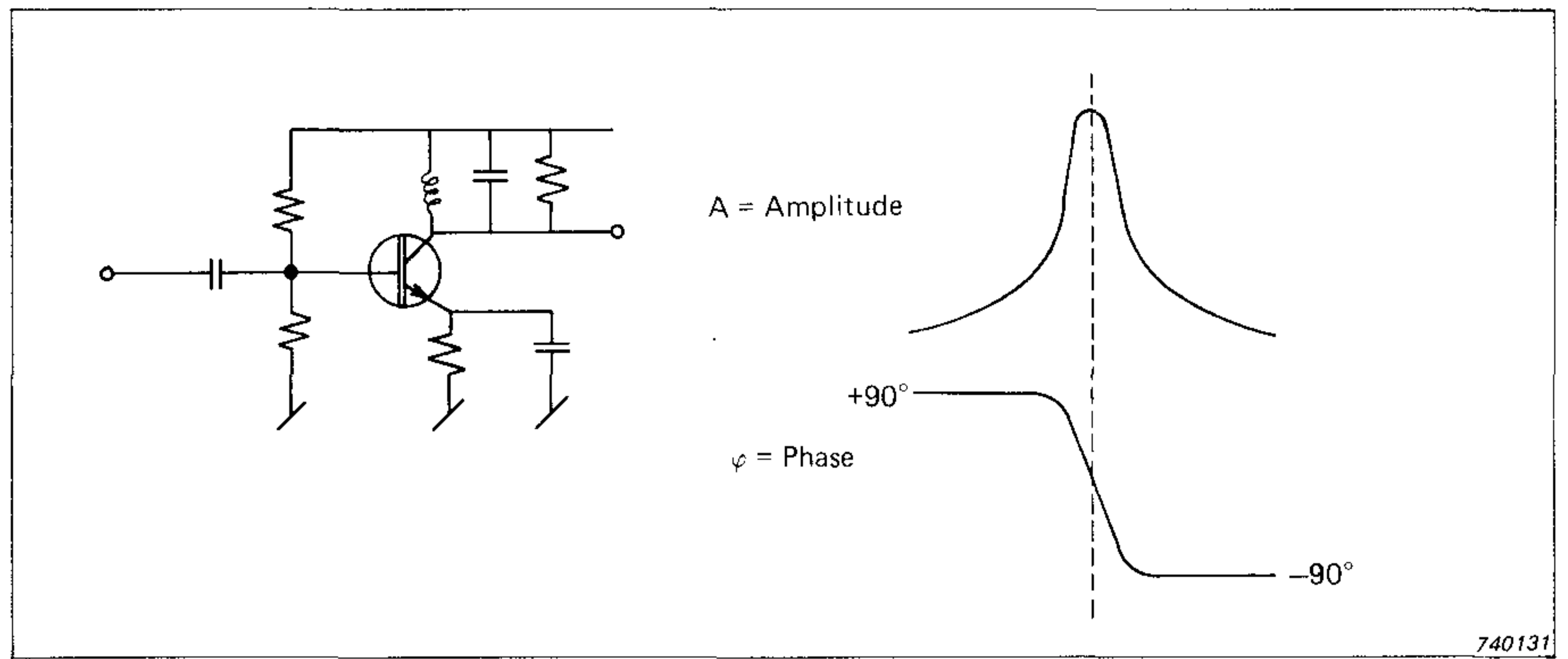
Fig. 26. Amplitude and phase response for band-pass filter
