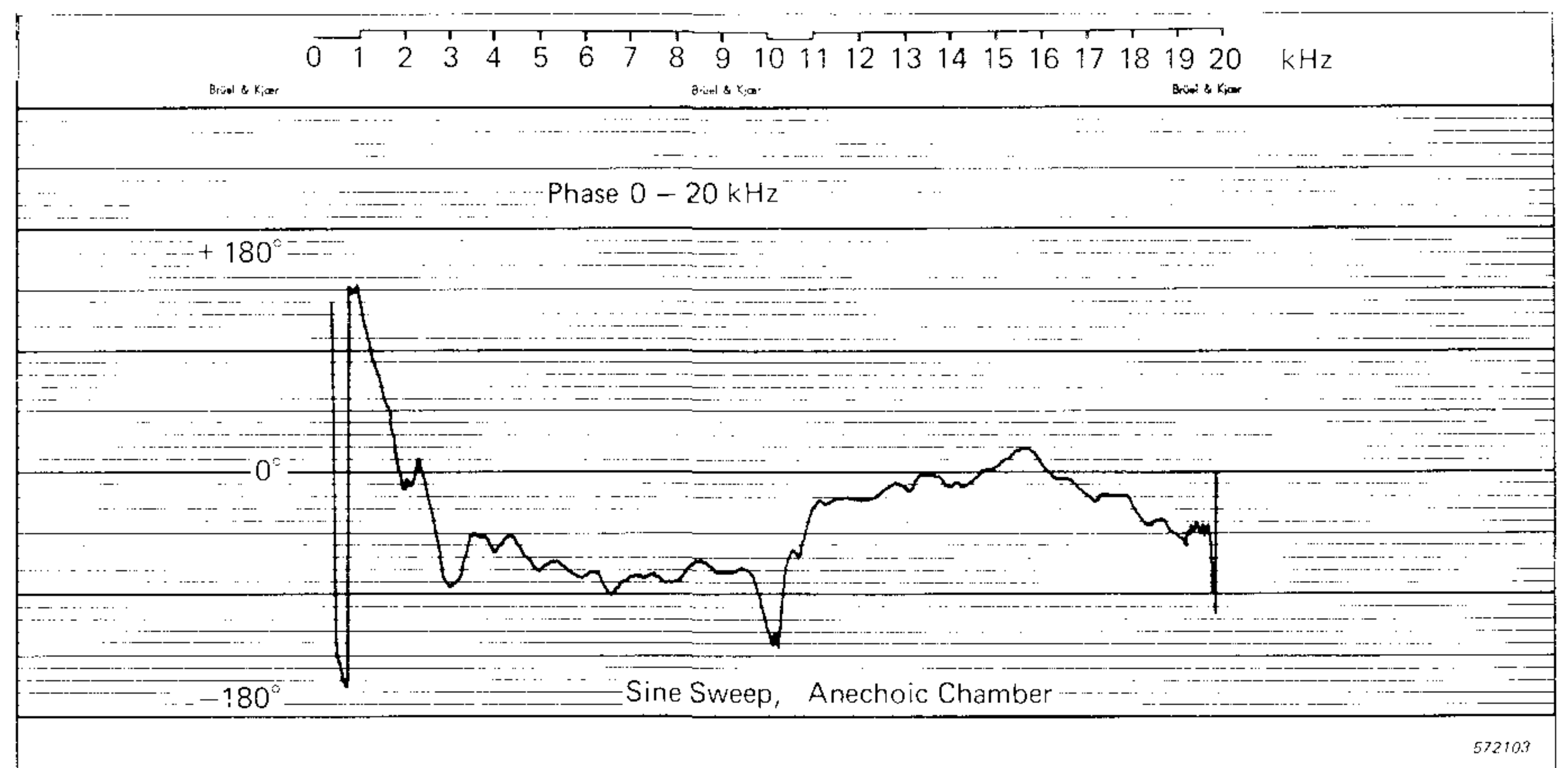
Fig.6. Typical phase response curve
