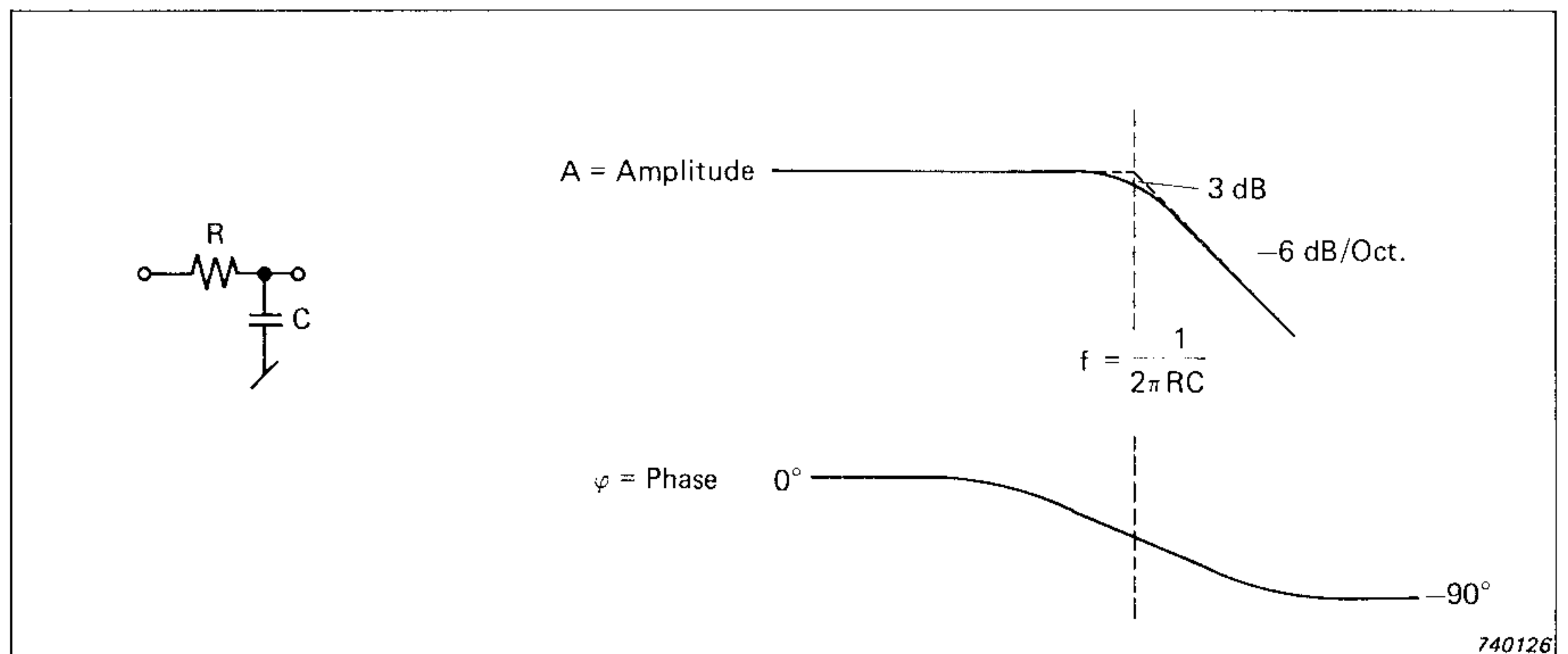
Fig.20. Amplitude and phase response for low-pass filter
