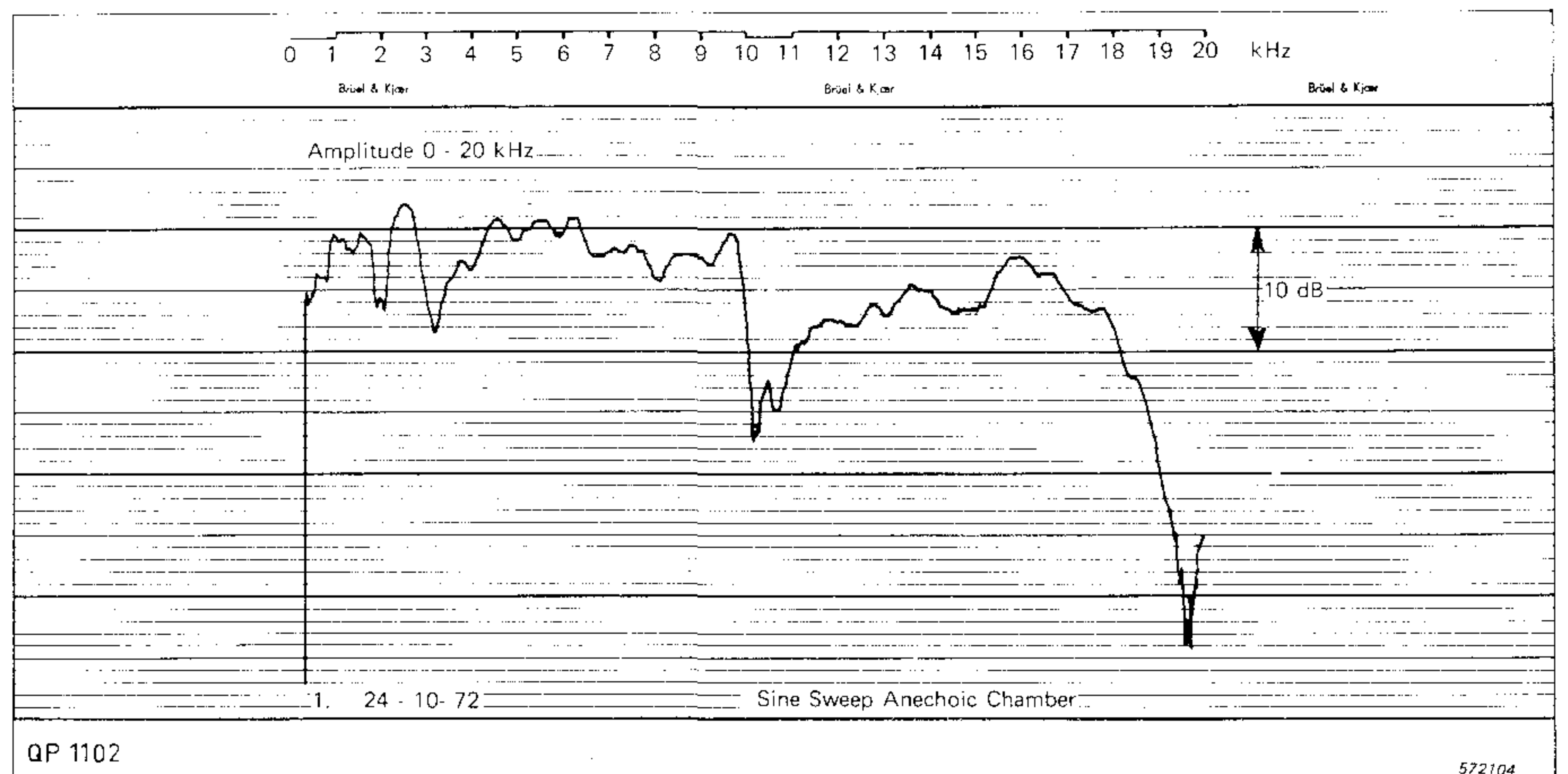
Fig.5. Typical amplitude response curve
