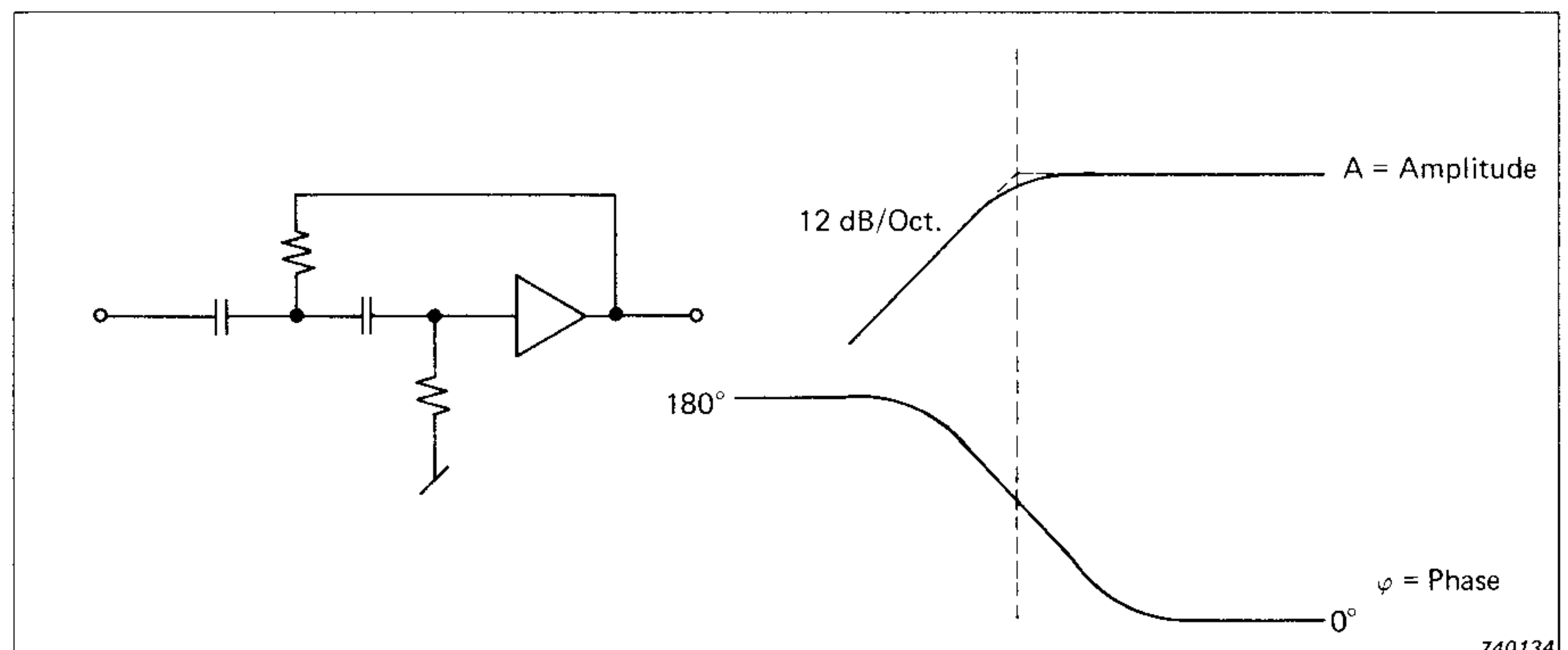
Fig.21. Amplitude and phase response for high-pass filter
