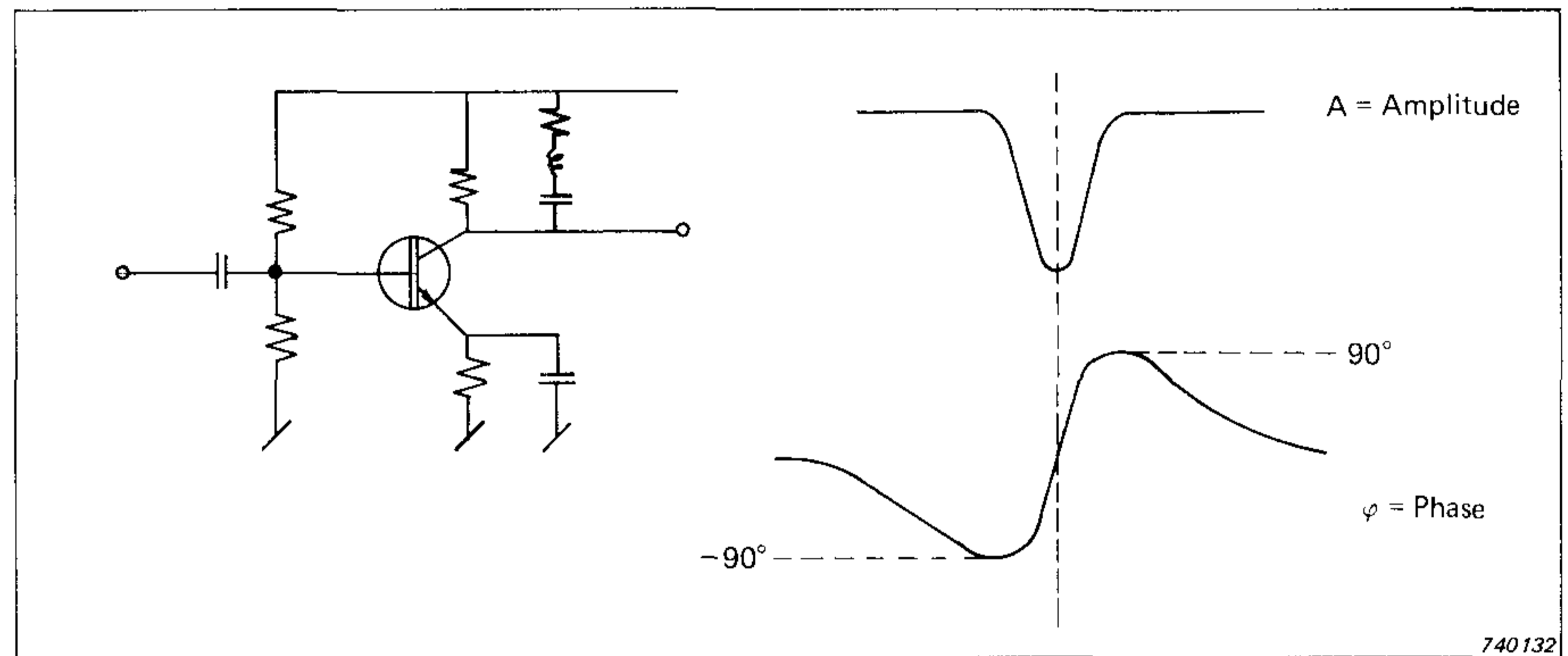
Fig. 27. Amplitude and phase response for band-stop filter
