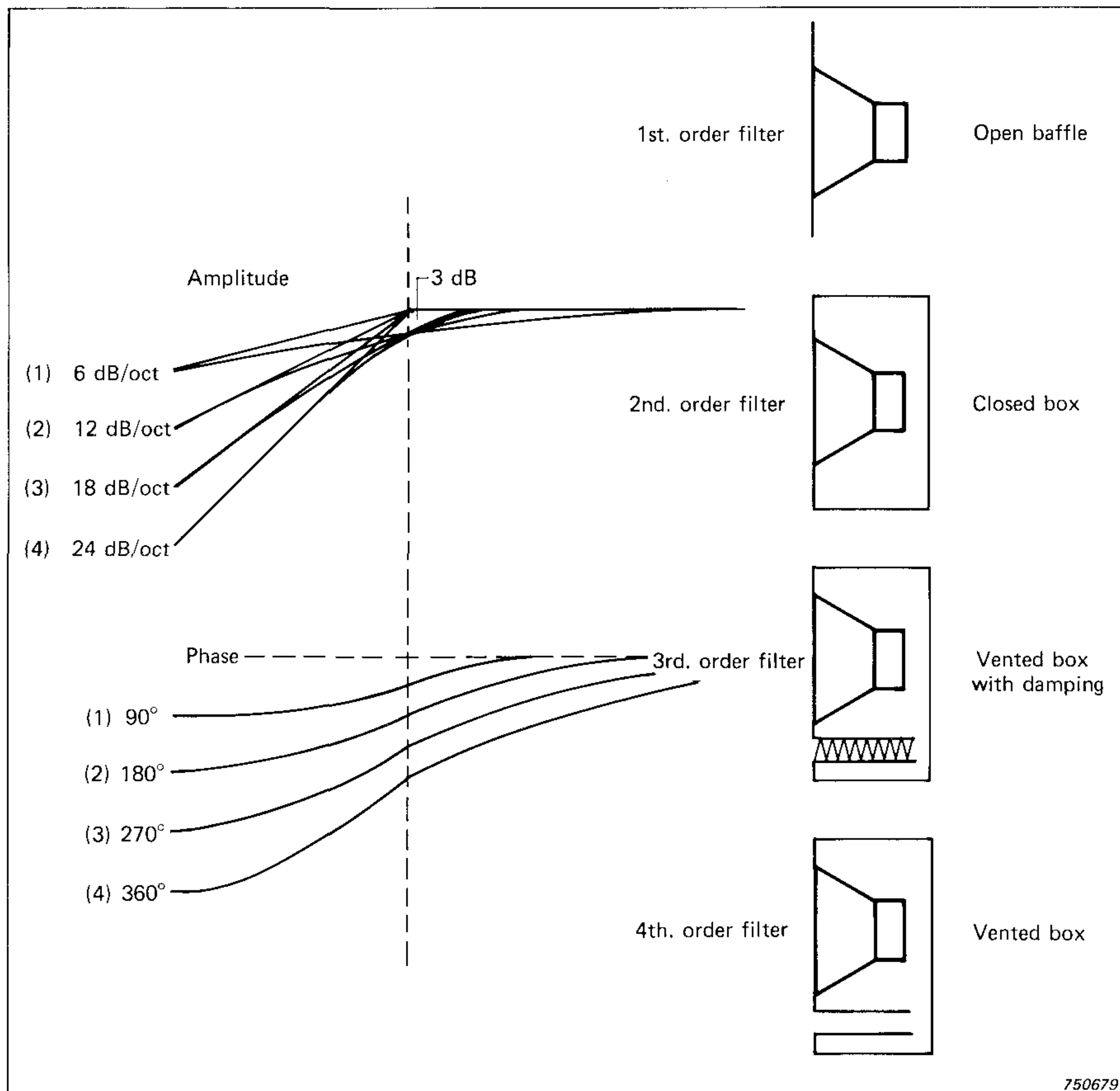
Fig.34. Corresponding amplitude and phase responses of conventional loudspeaker systems. Higher order filters introduce better amplitude response but worsen the phase response
