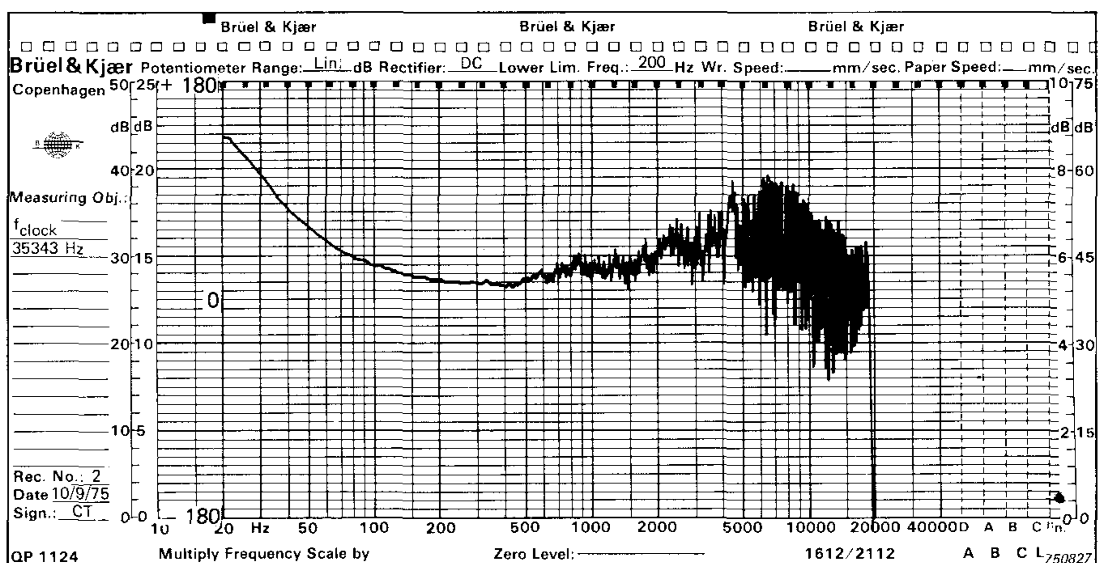
Fig.11. Tape recorder phase measurements using properly adjusted clock frequency
