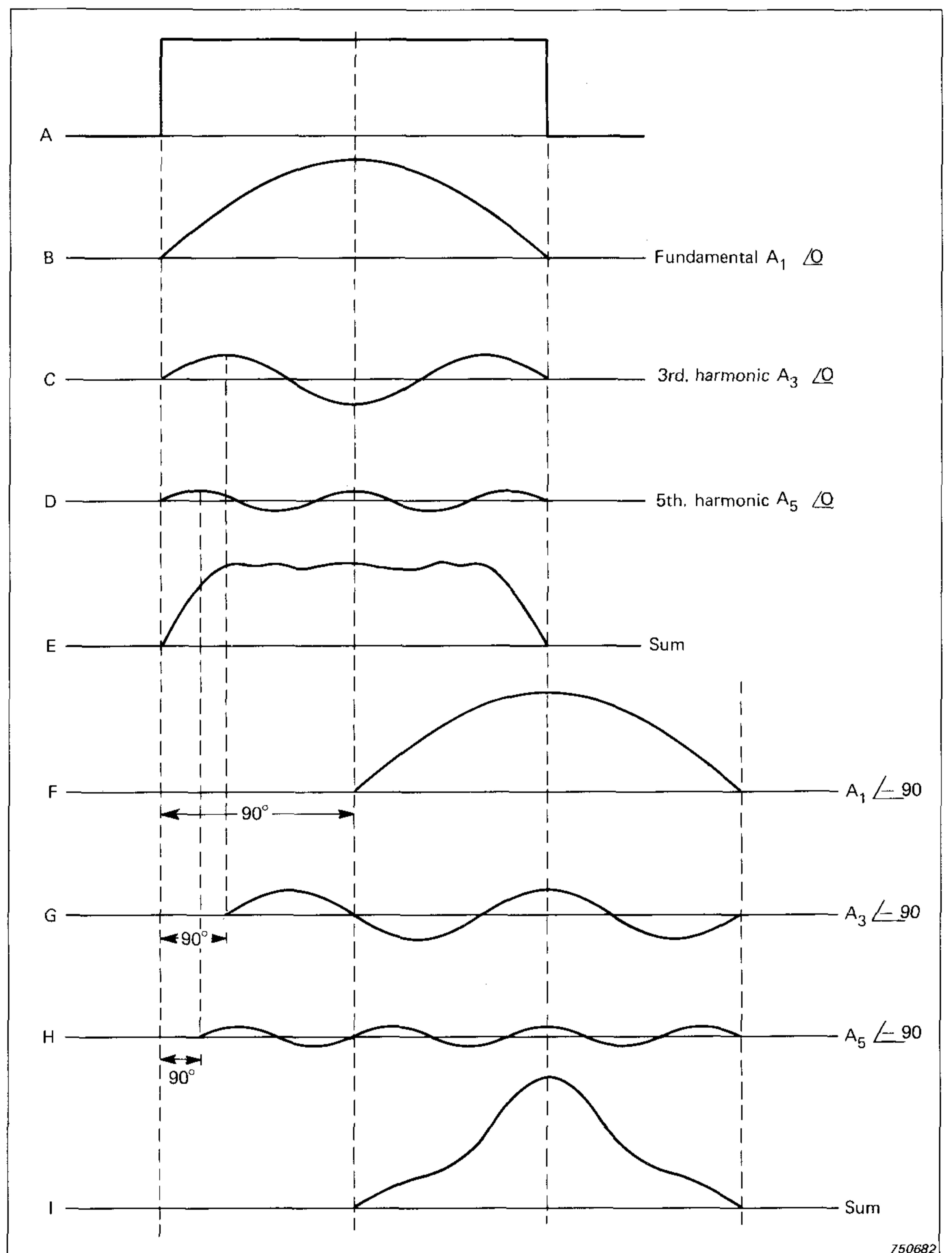
Fig. 2. A "continuous transient" a square wave consists of a fundamental sine wave and a number of harmonic components. When in phase (B-D) these can recombine (E) almost as the original signal (A). When shifted 90^\circ (F-H) the recombined signal (I) is very different from the original. Good transient response requires that the components are in phase
