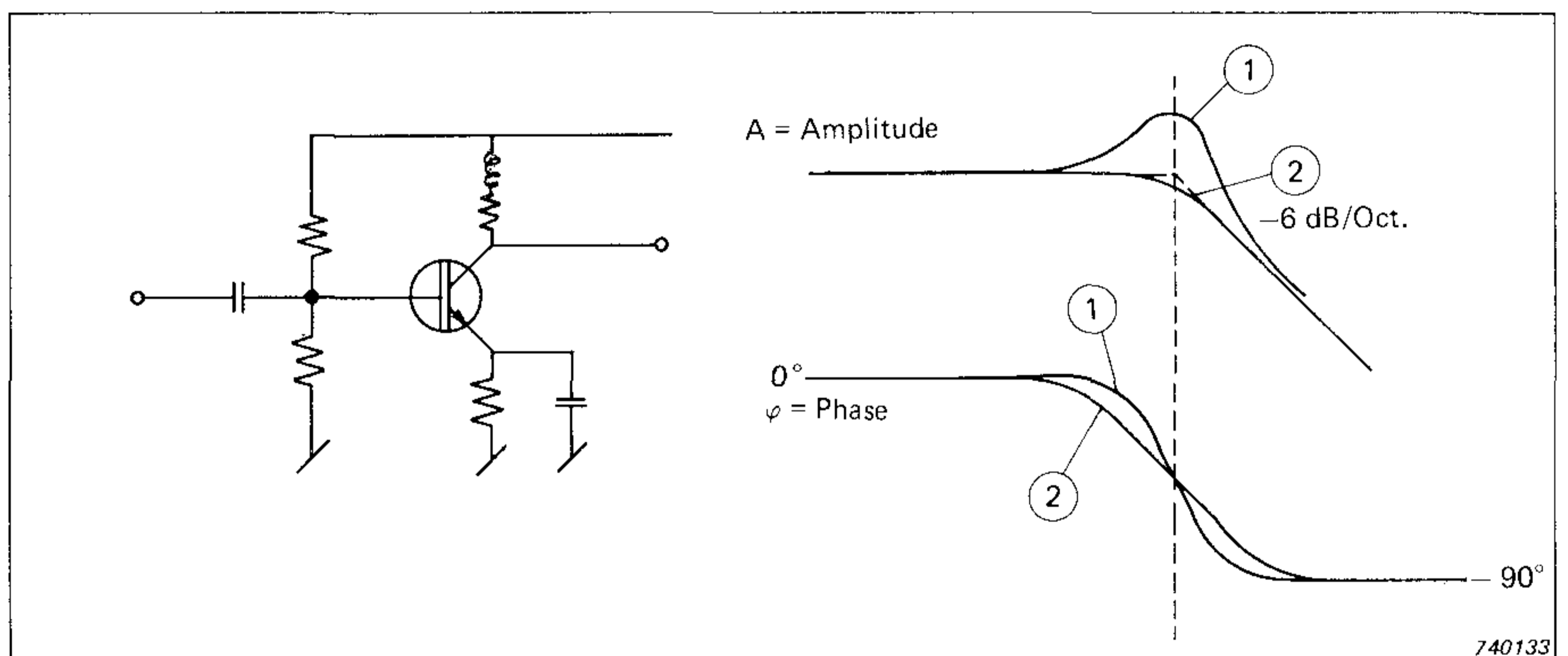
Fig. 28. Amplitude and phase response for low-pass configurations
